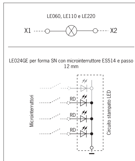
Fig. 5: Collegamento spie LED
